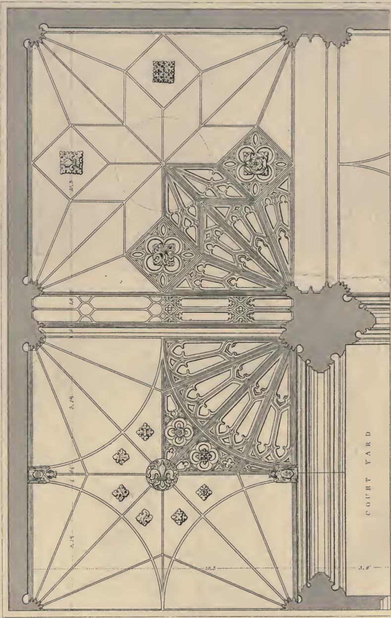
TWO COMPARTMENTS SOUTH EAST ANGLE CLOISTER OF ST STEPHEN'S CHAPEL.
